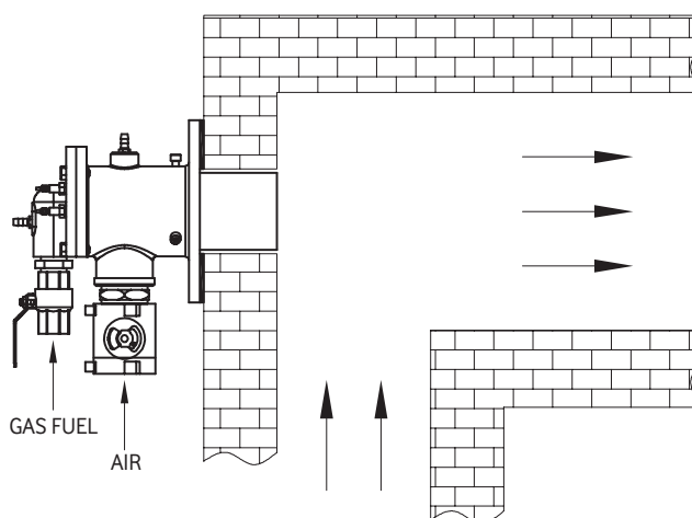
HOT GAS GENERATOR
