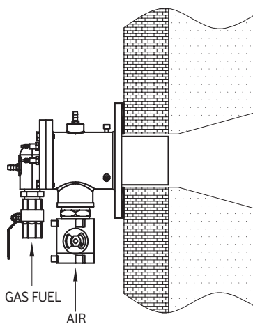
INDUSTRIAL FURNACE AND KILN APPLICATIONS WITH OPEN FIRING, CONICALLY OPENING COMBUSTION CHAMBER
