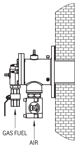
INDUSTRIAL FURNACE AND KILN INSTALLATIONS WITH OPEN FIRING, CYLINDRICAL COMBUSTION CHAMBER
