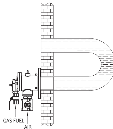
RADIANT TUBE HEATING
